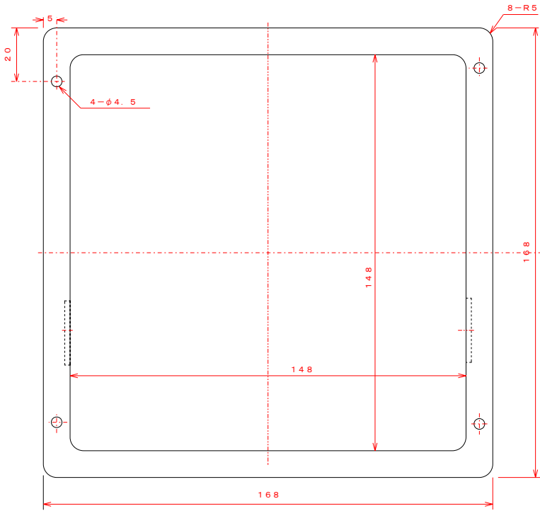
埋め込み金具 FR-21 材質SUS t=2
